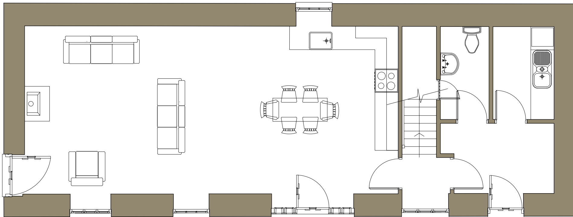
Ground Floor plan TRENDEAL BARN
